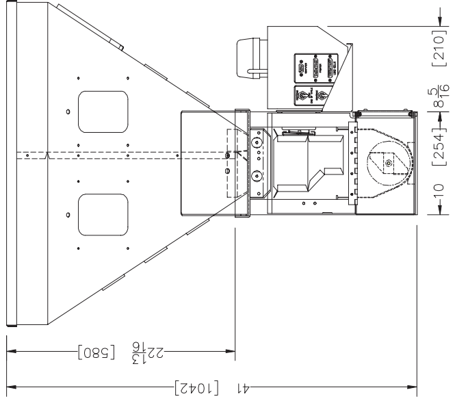
WSB 140 FRONT VIEW
