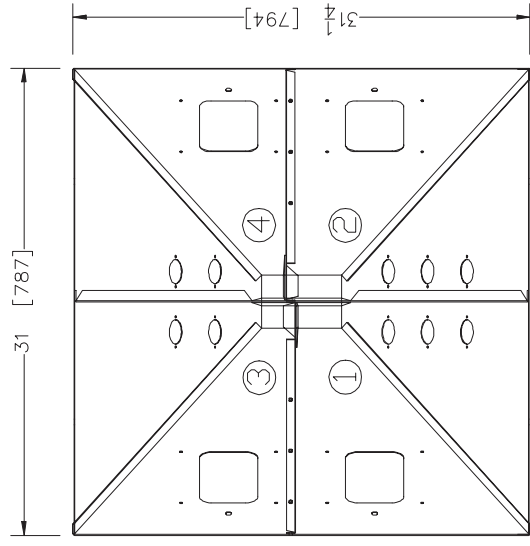
WSB 140 HOPPER TOP VIEW Controller Side
