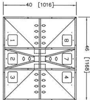
CONTROLLER SIDE
