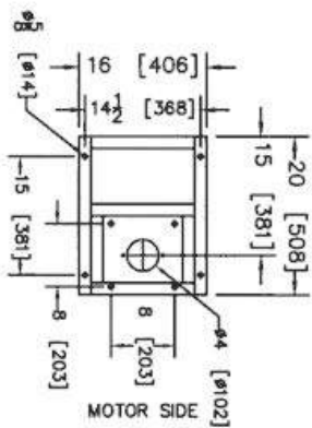
FOOTPRINT
