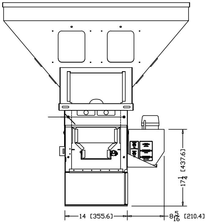
WSB 240 FRONT VIEW
