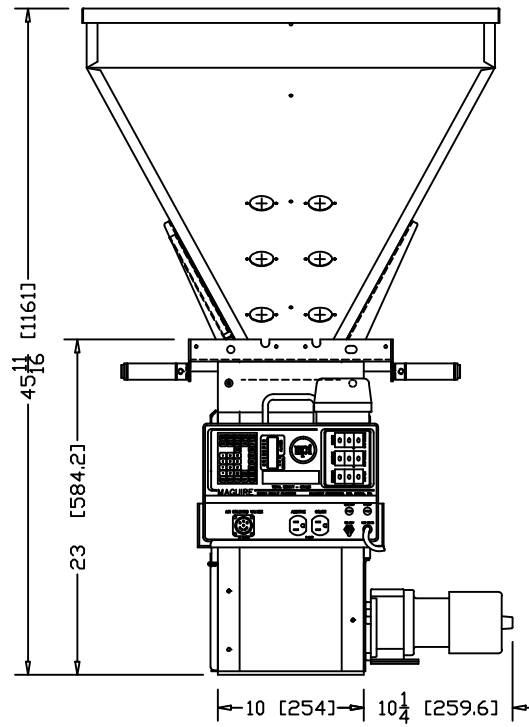
WSB 240 SIDE VIEW
