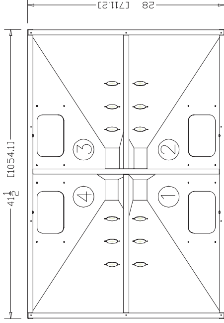
WSB-240 HOPPER TOP VIEW
