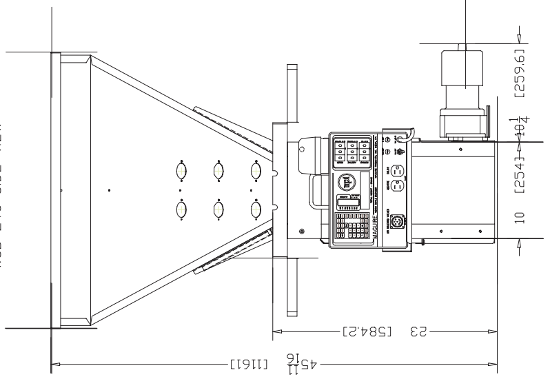
WSB 240 SIDE VIEW
