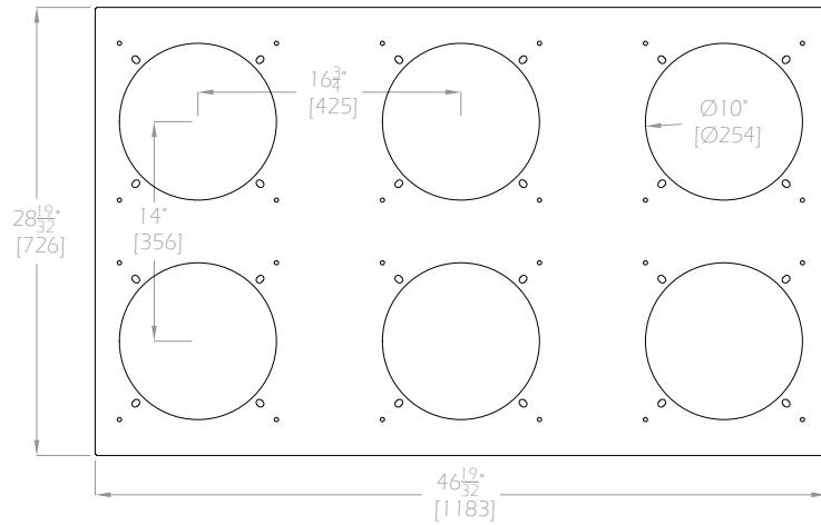
WXB-260 FRONT VIEW
