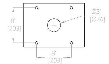
WXB-260 Footprint
