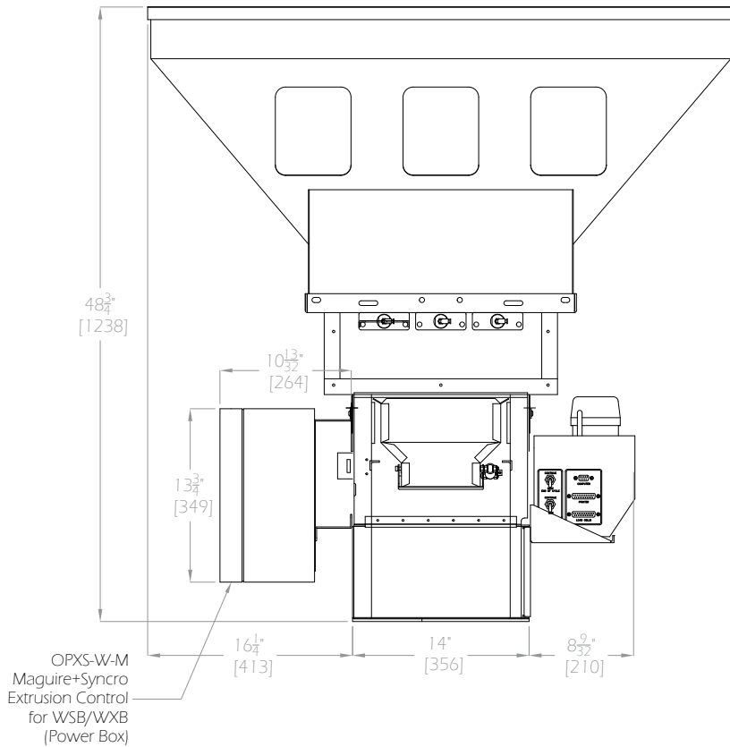
WXB-260 FRONT VIEW
