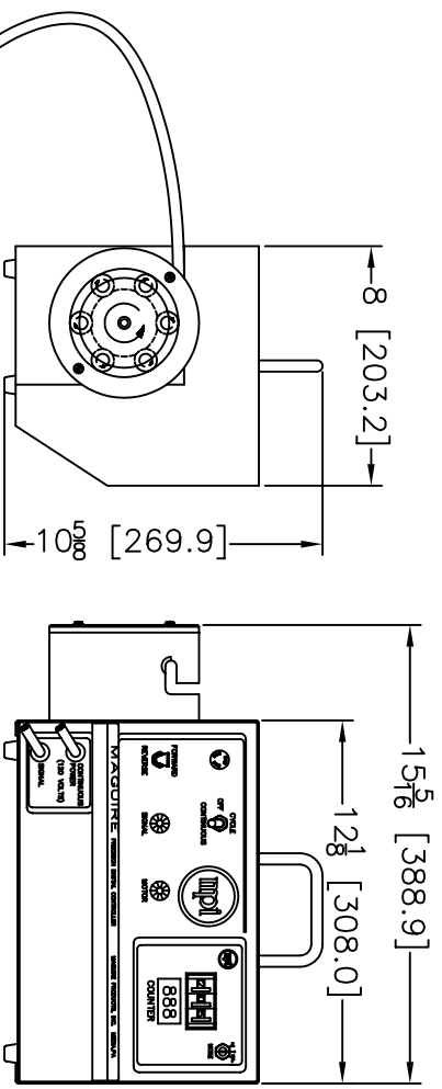
MPA-6 Six-Roller Liquid Color Pump
