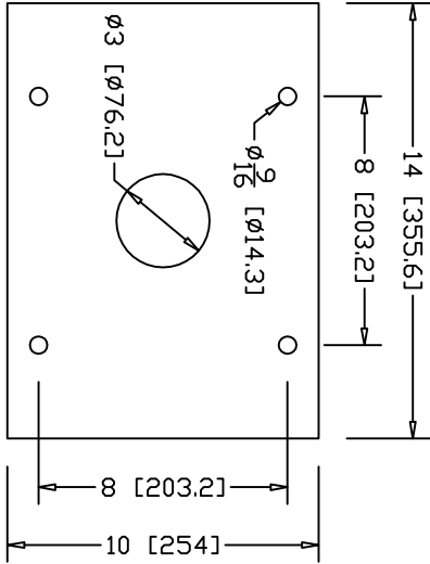
MPM-18 TOP PLATE & FOOTPRINT ¼" [6.4mm] STEEL PLATE
